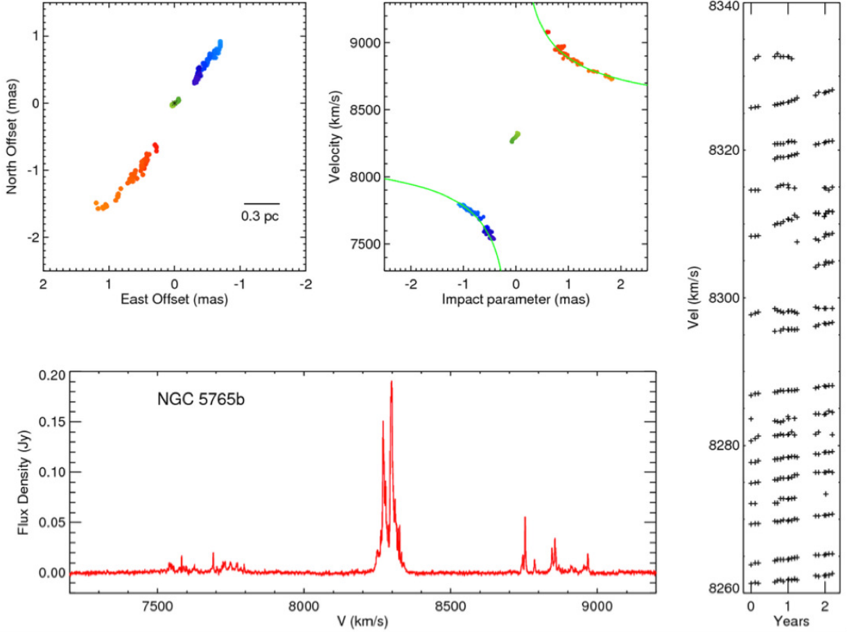
Figure 1: A summary of observations of the H 2 O megamaser in NGC 5765b (also see [4]). These observations determine the galaxy’s distance of 126.3 \pm 11.6 Mpc. The top left panel shows the VLBI maser map, with colors of the maser spots representing the line-of-sight velocities. The top center panel shows a position-velocity (P-V) diagram. The impact parameter represented on the x -axis is the angular distance measured along the length of the edge-on disk. The solid green lines on the P-V diagram represent a Keplerian fit to the rotation curve. The bottom panel shows a representative GBT spectrum. Masers in edge-on AGN accretion disks have a characteristic profile with three groups of maser features, evident in this spectrum. The features centered near 8300 \text{ km s}^{-1} originate from the front side of the edge-on disk while those centered near 7650 \text{ km s}^{-1} and 8850 \text{ km s}^{-1} originate from the midline of the disk on the approaching and receding sides, respectively. The right panel shows results of GBT spectral monitoring. Each symbol on the plot marks the velocity of a maser peak in the systemic part of the spectrum. The maser velocities increase with time according to the centripetal acceleration of maser clouds as they orbit the central supermassive black hole.
